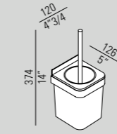
AMEM855_ Porta scopino/ Toilet brush holder
