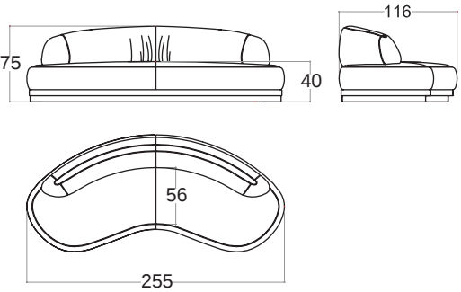
GLAMIS SOFA DIVANO GLAMIS
